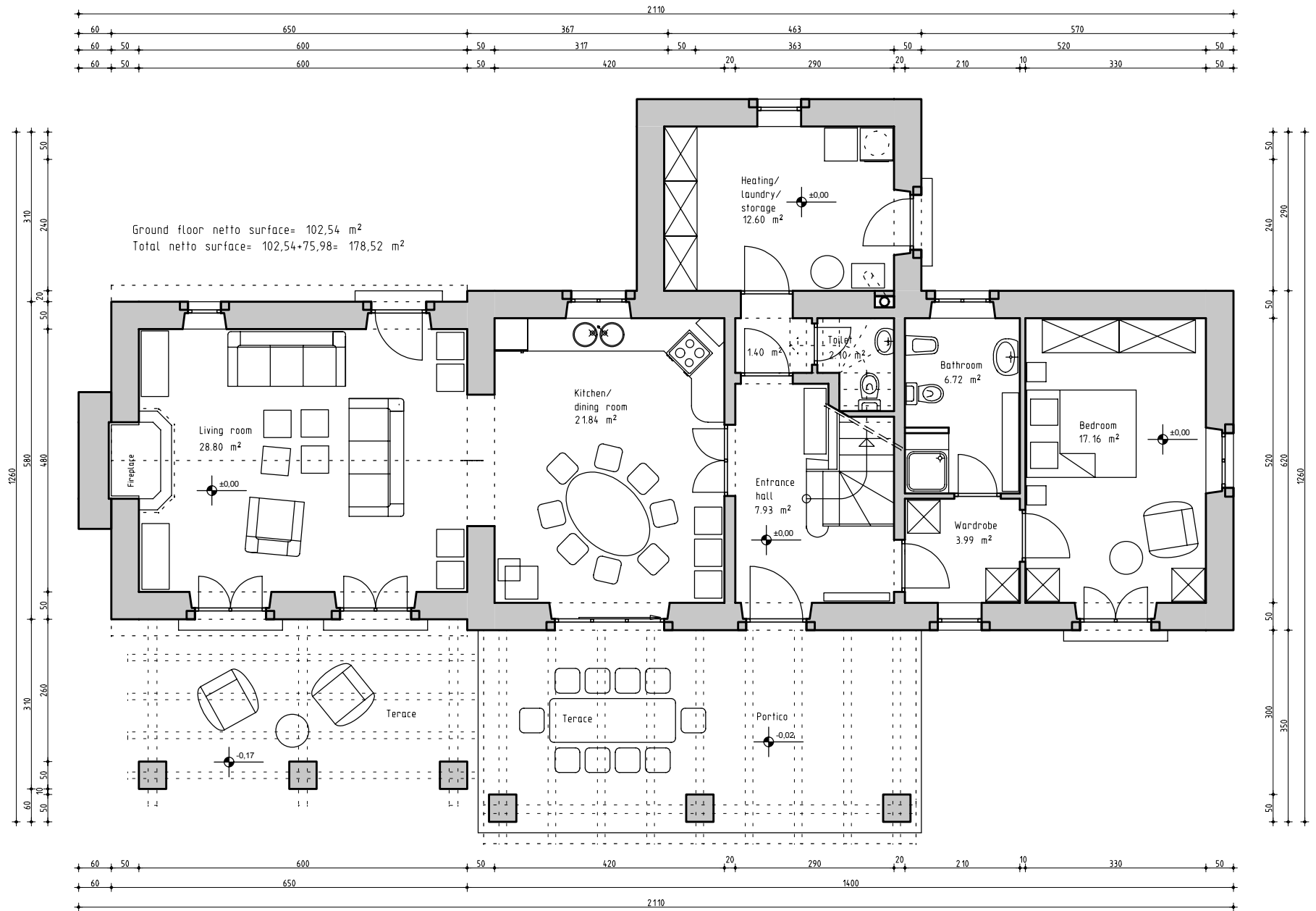
Sovinjak Villa 1 Ground floor Scale 1:100
